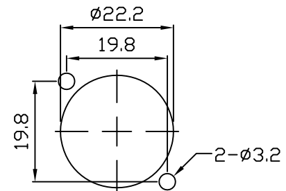
PANEL CUT OUT(±0.05) (FRONT SIDE)
