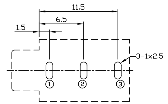
PCB LAYOUT(±0.05) (TOP VIEW)
