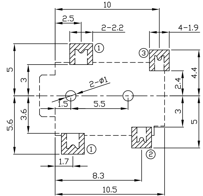
RECOMMENDED PCB LAYOUT TOLERANCE: \pm 0.05 (TOP VIEW)
