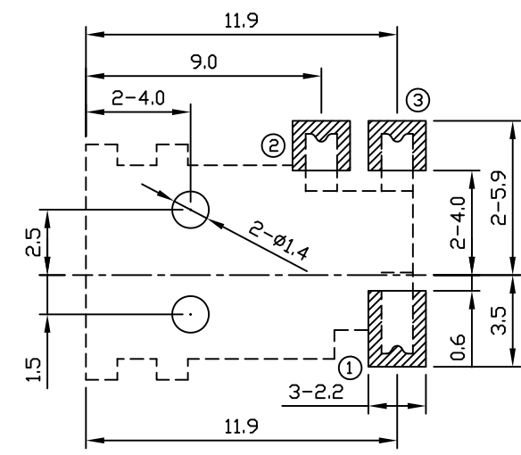
RECOMMENDED PCB LAYOUT TOLERANCE: ±0.05 (TOP VIEW)
