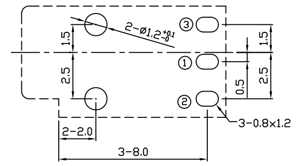
RECOMMENDED PCB LAYOUT TOLERANCE: ±0.05 (TOP VIEW)
