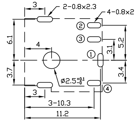
RECOMMENDED PCB LAYOUT TOLERANCE:±0.05 (TOP VIEW)
